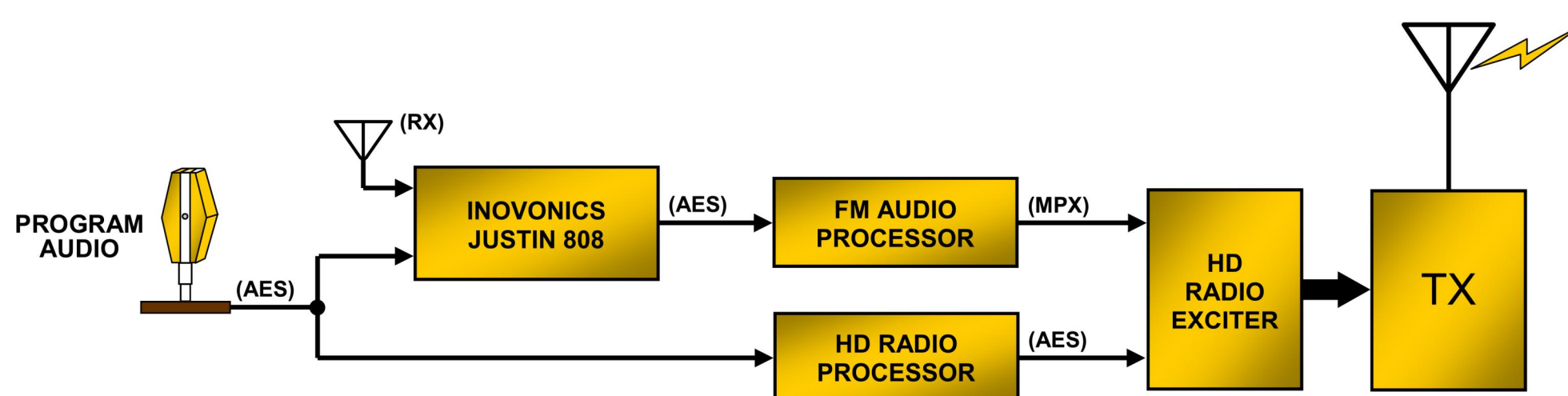
JUSTIN Implementation in FM Air Chain With Dual Audio Processors
