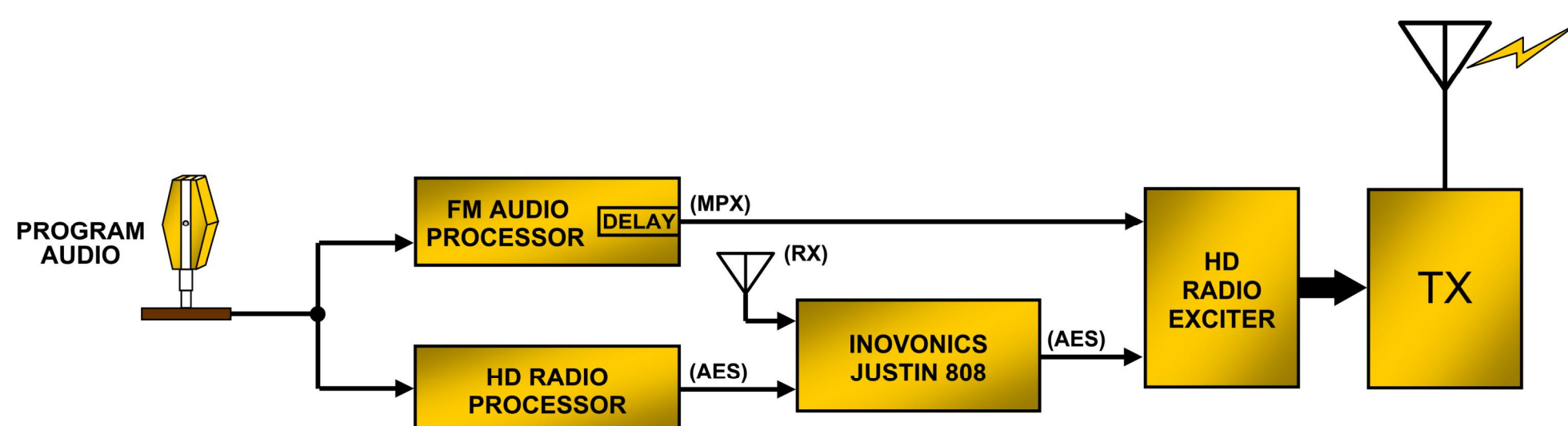
JUSTIN Implementation in HD Radio Air Chain With Dual Audio Processors
