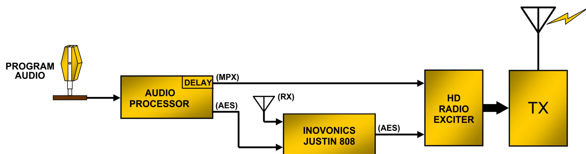
JUSTIN Implementation in HD Radio Air Chain With Single Audio Processor
